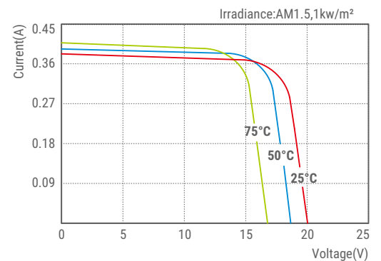
SLP005S-12U I-V Curves
